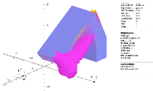
Figure 5: OPERA3d/ELEKTRA calculation result of the eddy current distribution in the iron of the sextupole magnet.
