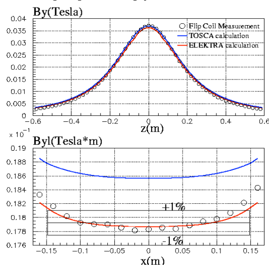
Figure 1: Top figure shows the y component of the magnetic field, B_y , by the steering magnet CHN along the z axis. The bottom figure shows the integral of the y component of the magnetic field, B_{yl} , with respect to z between -0.6 m and 0.6 m as a function of x at y=0 m. Flip coil measurements are shown in open circles, TOSCA calculation in the blue line and ELEKTRA calculation in the red line.
