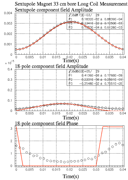
Figure 6: The sextupole component of the sextupole magnet in the long coil as a function of time from the current minimum timing (top figure). The 18-pole component in the long coil (center figure). The relative phase of the 18-pole component (bottom figure). Measurement results are shown in circles and the ELEKTRA calculation are shown in red lines.
