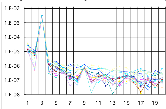
Figure 4: Amplitude of the harmonic components of the magnetic field flux in the long coil. Data were taken and shown for six times each for three sextupole magnets.
