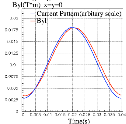
Figure 3: The field integral B_{yl} as a function of time is shown in the red line and the arbitrary scaled current pattern is shown in the blue line. The field integral B_{yl} delayed 0.7 ms from the current pattern.
