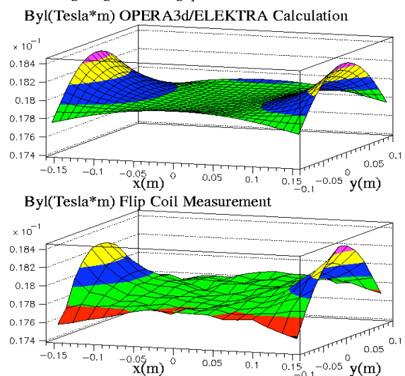
Figure 2: The top figure shows the ELEKTRA calculation of the integral of the y component of the magnetic field with respect to z between -0.6 m and 0.6 m, B_{yl} , by the steering magnet CHN as a function of x and y. The bottom figure shows the flip coil measurement of the field integral B_{yl} .
