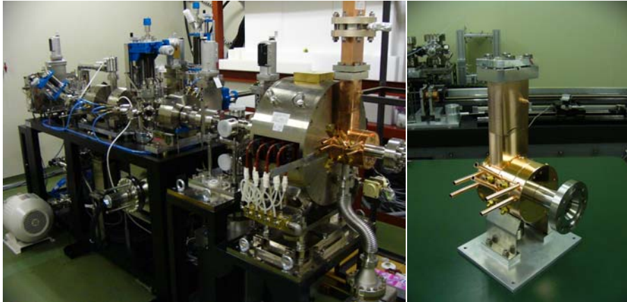
Figure 1: Photocathode femtosecond rf gun and electron diffraction measurement system
