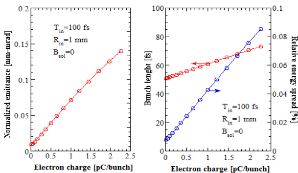
Figure 5: Normalized transverse emittance, bunch length and energy spread versus bunch charge.
