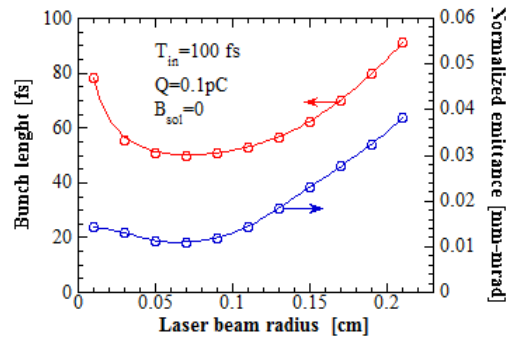
Figure 3: Bunch length and normalized transverse emittance versus laser spot radius.
