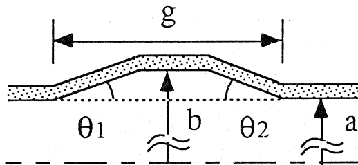
Figure 1. Parameters to show the dimension of the structures.
