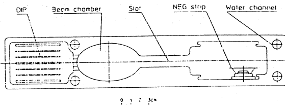
Figure 2. The vacuum chamber cross section
