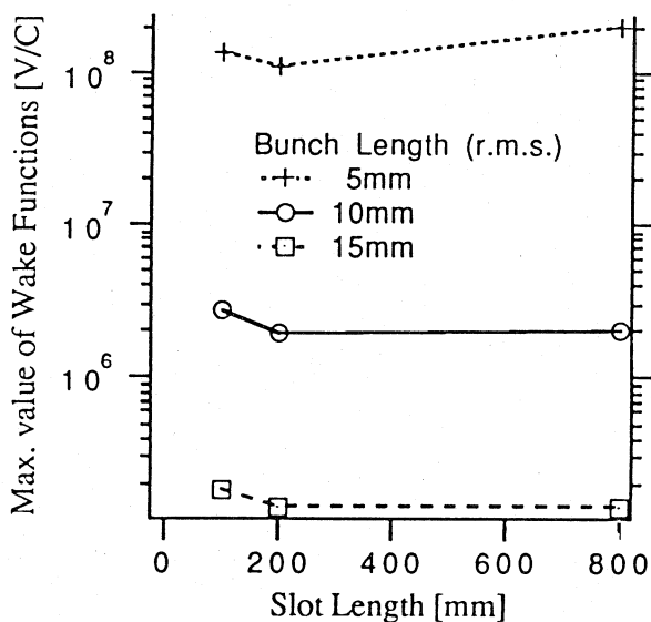
Figure 5. Wake Function vs..Slot Length
