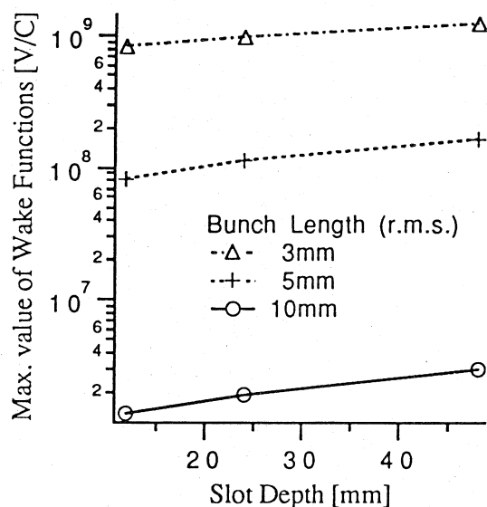
Figure 6. Wake Function vs..Slot Depth
