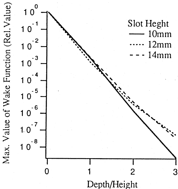
Figure 4. Wake Function vs. Depth / Height of the slot for different height(from ref. [3])
