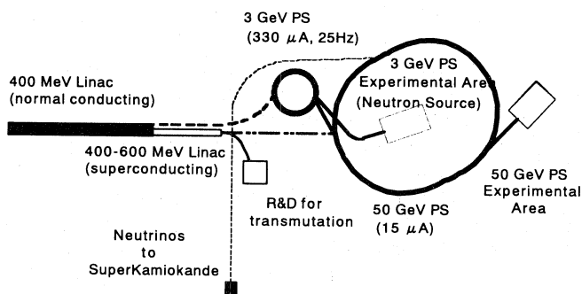
Fig. 1 Layout of the accelerator complex of the Joint Project.
