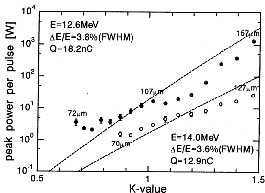
Figure 1: Peak power of SASE measured as a function of K-value of the wiggler. The solid and the open circles denote the measured data points for the beam energy of 12.6 and 14.0 MeV, respectively. The dashed lines were theoretical values predicted by one-dimensional model. See text for details.
