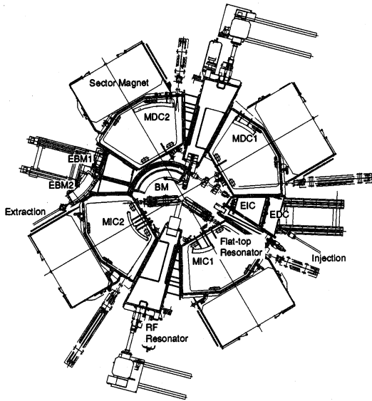
Figure 4: Plan view of the IRC.
