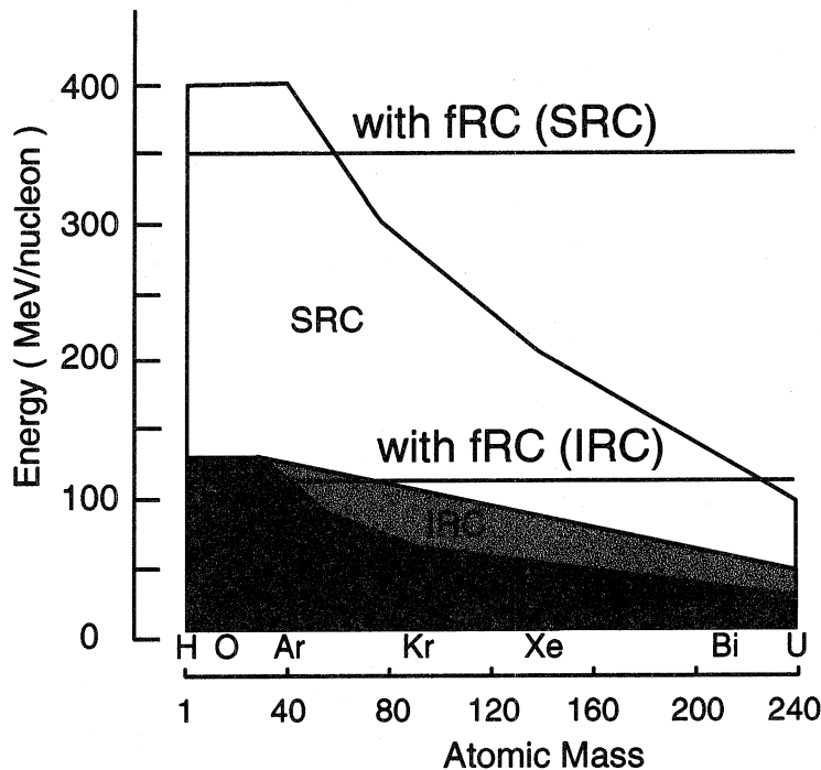
Figure 3: Energy vs. mass performance of RIBF accelerator complex.
