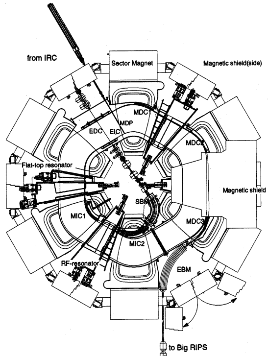
Figure 5: Plan view of the SRC.
