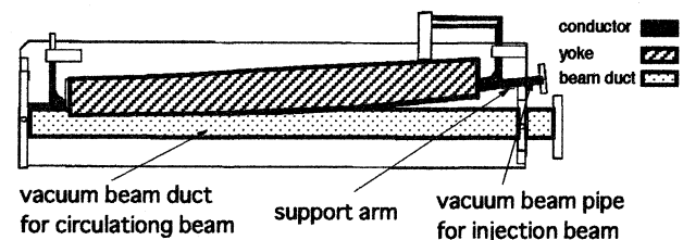
Figure 1: Flat view of the septum. The beam runs from the right to the left. The upper side, that was an outer side of the ring, is a vacuum pipe for the injected beam and the lower side is the beam duct for the circulating beam.
