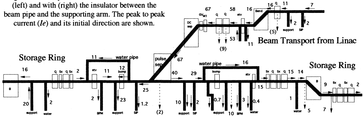
Figure 6: The septum induced AC current with the insulator of the beam pipe.
