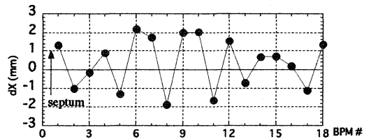
Figure 3: Example of horizontal closed orbit distortion around the ring produced by an error kick at the location indicated by the arrow.
