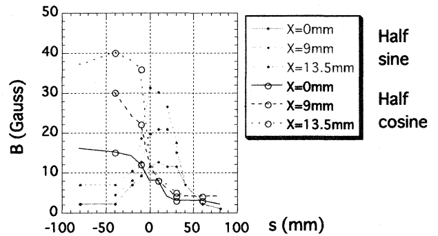
Figure 8: Distribution of the stray field. We defined x=0 at the designed centre of the circulating beam, where the wall of the vacuum duct is at x=21 mm. The septum exists at s<0 and ends at s=0 . The thick lines are cosine-like components and the thin lines are sine-like components of the stray field.
