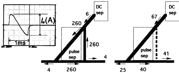
Figure 5: The septum induced AC current without (left) and with (right) the insulator between the beam pipe and the supporting arm. The peak to peak current ( I_e ) and its initial direction are shown.
