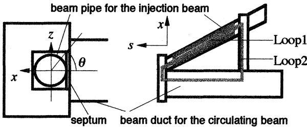
Figure 2: Schematic view of the pulse septum which shows three possible current loops.
