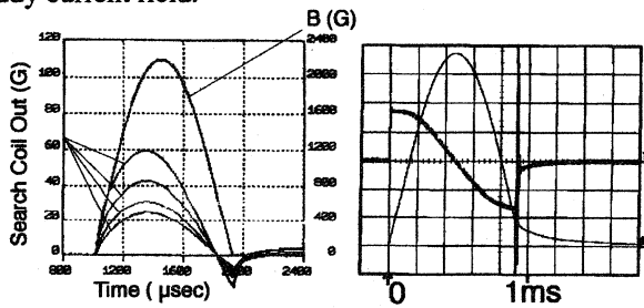
Figure 7: The pulse shapes of the induced voltage at the search coil without (left) and with (right) the insulator. In the left main magnetic field and the integrated shape of the search coil voltage (=current) is shown. In the right the cosine-like shape was the induced voltage and the sine-like shape was the integration of the voltage.
