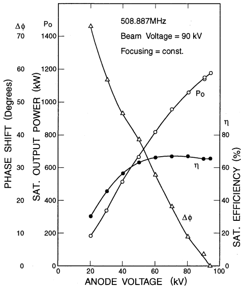
Figure 3: Performance as a function of anode voltage.
