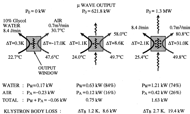
Figure 7: Hybrid cooling system of klystron output window.
