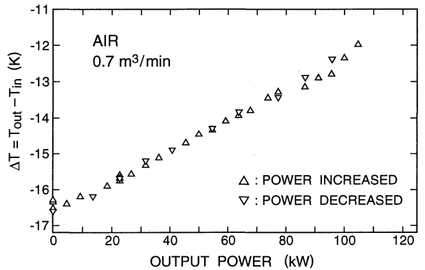
Figure 5: Compensated temperature rise of air as a function of klystron output power.
