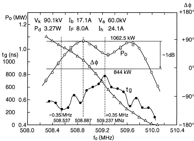
Figure 4: An example of instantaneous bandwidth characteristics of T41. The beam voltage, V_k , is 90.1 kV.
