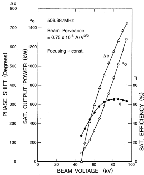
Figure 2: Performance of T41 as a function of beam voltage.
