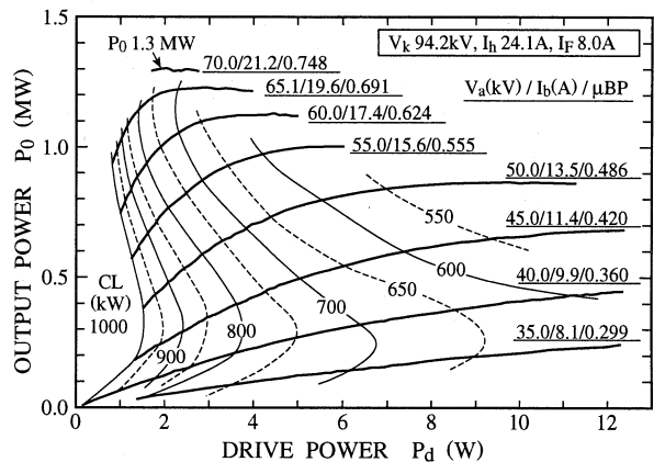
Figure 1: Klystron characteristics at KEKB frequency, 508.887 MHz. Constant collector loss curves (in kW) are shown up to 1000 kW. The highest rf output is 1.3 MW.
