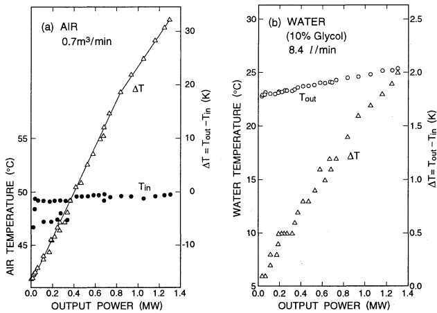
Figure 6: Temperature rise of (a) cooling air and (b) chiller cooling water containing 10% ethylene glycol as a function of klystron output power up to 1.3 MW.
