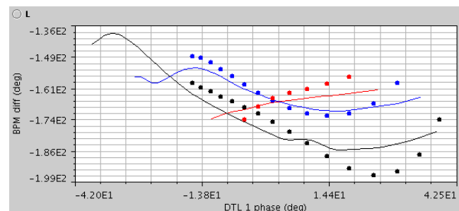
Fig.1. Phase difference between two BPMs downstream of Tank 1, vs. tank 1 klystron phase. Dots are model results, curves are measured data. Blue = nominal amplitude setting, red = 95%, black = 105%.
