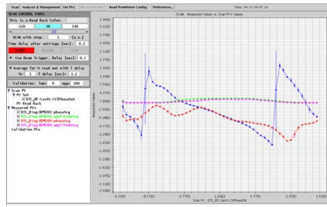
Fig. 6. Example use of the 1-D scan application, varying a klystron phase and monitoring BPM phases and amplitudes.
