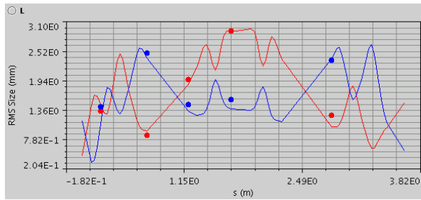
Fig.2. Beam size along the MEBT section. Dots are measured values and the curves are model predictions after solving for the initial Twiss parameters. Red = horizontal, blue = vertical.
