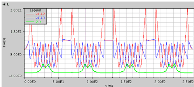
Fig. 3. Horizontal beta (red), vertical beta (blue) and dispersion (green) predicted by the online model for the SNS Ring.
