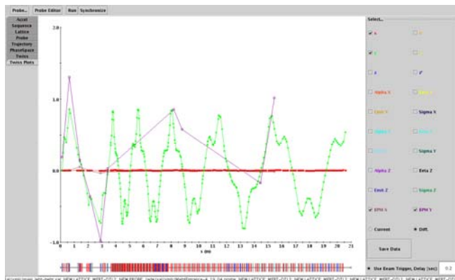
Fig. 5 The online model application run in the orbit difference mode - showing difference between the calculated position before and after a corrector change as well as the observed change in BPM positions.
