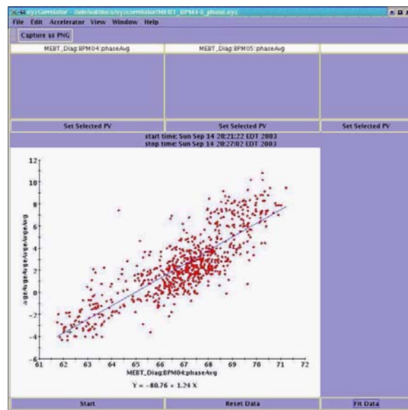
Fig. 7. The XYZ Correlator application running with 2 signals (phase signals from 2 BPMs).
