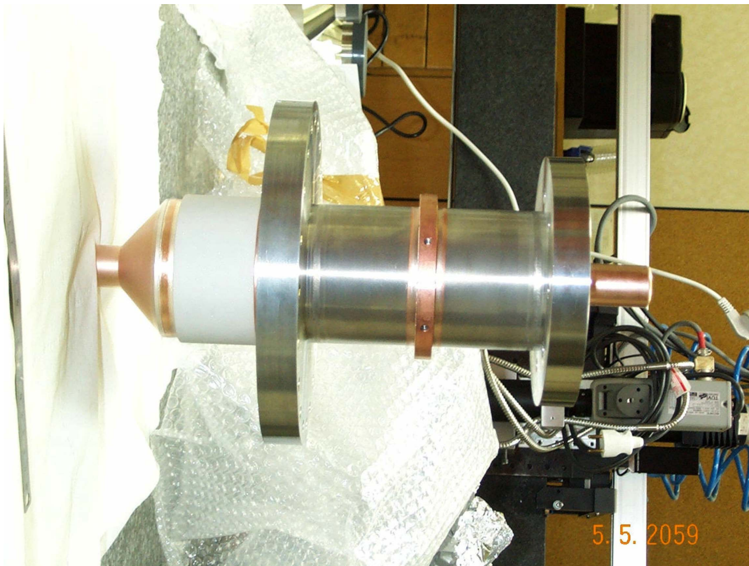
Cold coupler part (SNLS)
